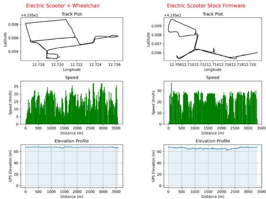
Figure 5.1. Distance traveled during the road test
