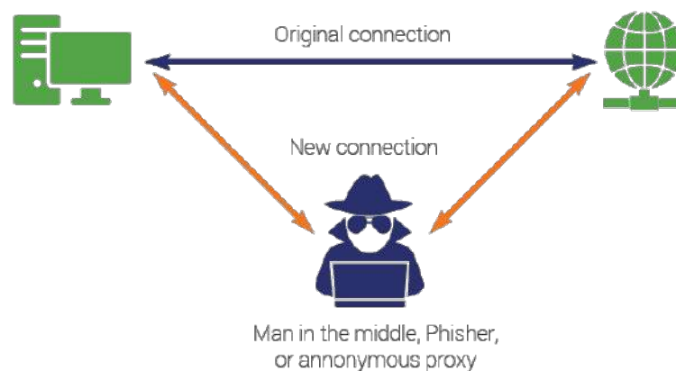
Figure 4.1. Man-in-the-middle attack
