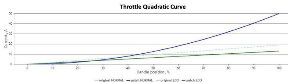
Figure 1.7. Throttle Quadratic Curve
