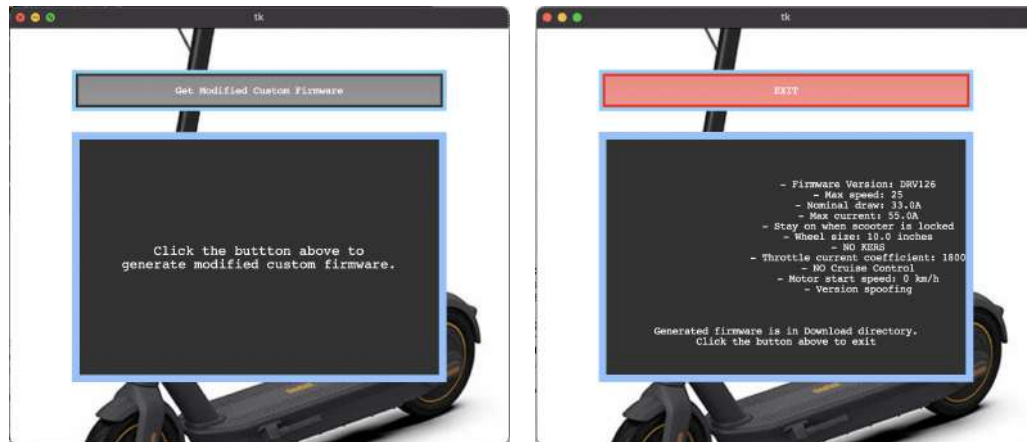
Figure 4.8. Graphical interface of the firmware generator
