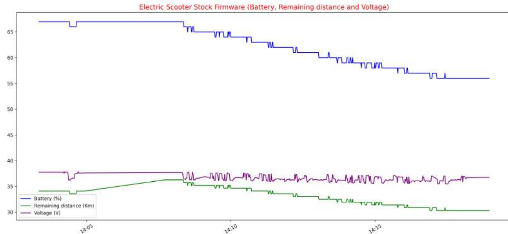
Figure 5.5. E-scooter, Battery, remaining distance and voltage over time
