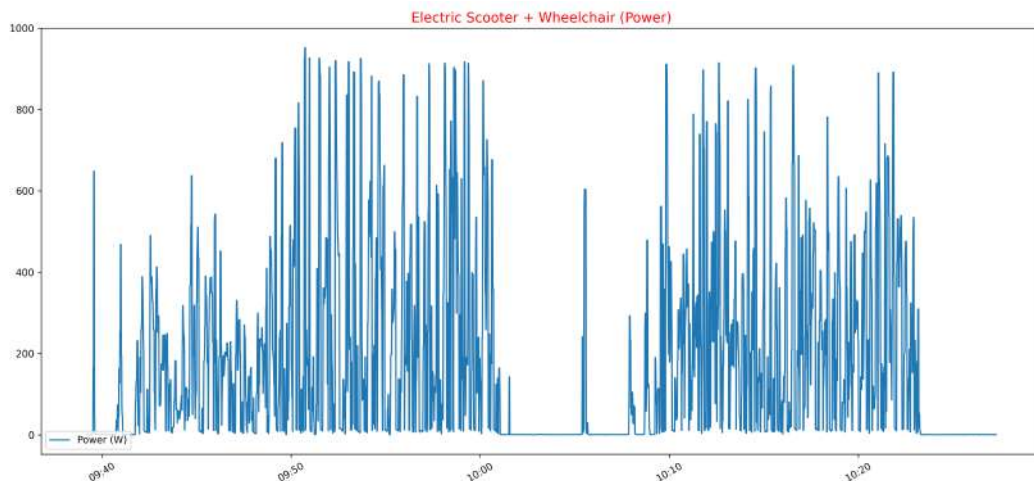
Figure 5.6. E-scooter + Wheelchair, Power over time
