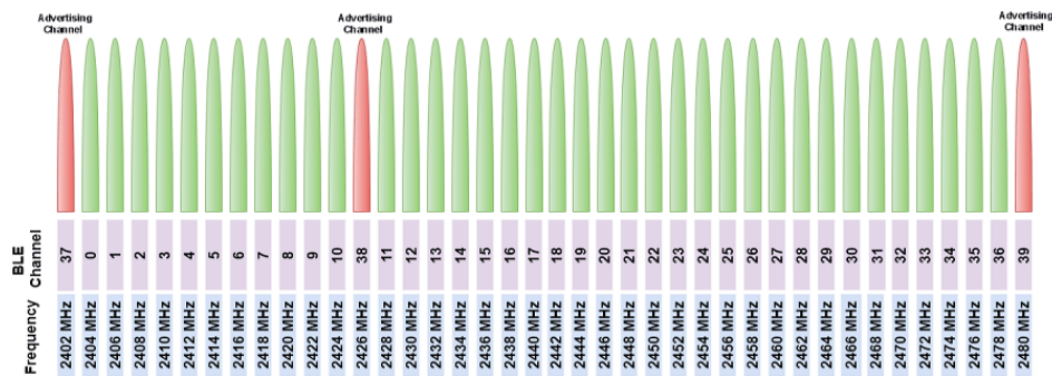
Figure 3.2. Frequency Band Bluetooth Low Energy
