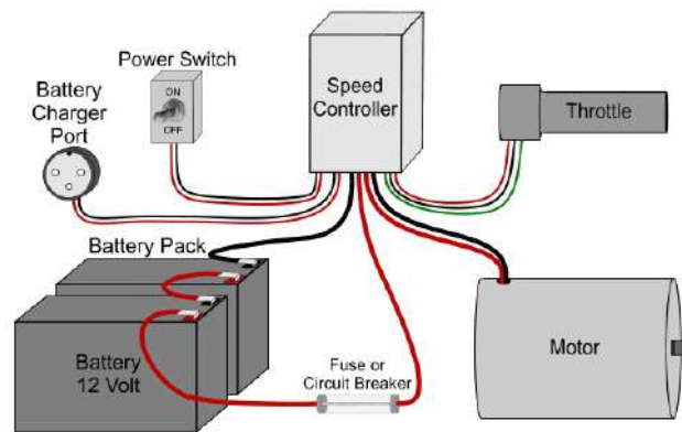
Figure 1.1. Electric Scooter Wiring Schematic
