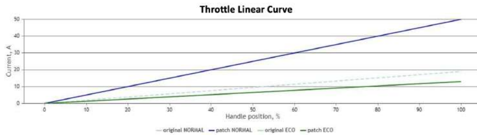
Figure 1.6. Throttle Linear Curve
