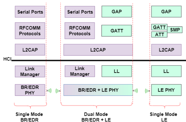
Figure 3.1. The architecture of the Bluetooth stack
