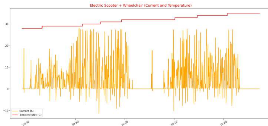
Figure 5.2. E-scooter + Wheelchair, current and temperature over time
