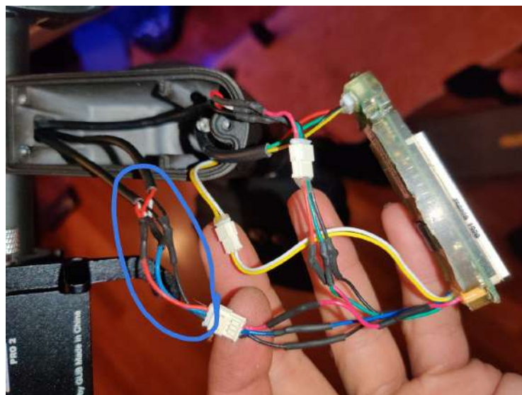
Figure 1.5. Brake lever connections
