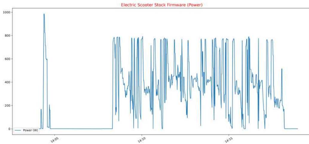
Figure 5.7. E-scooter, Power over time
