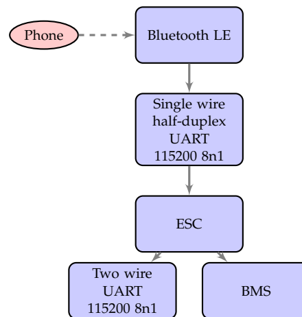
Figure 1.8. Xiaomi/Ninebot Protocol
