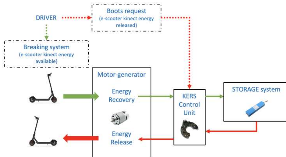
Figure 1.3. KERS functioning
