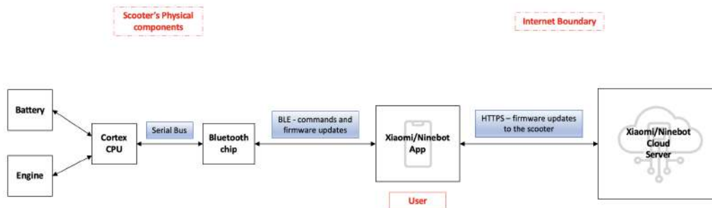
Figure 4.3. Scooter-App Communication Diagram
