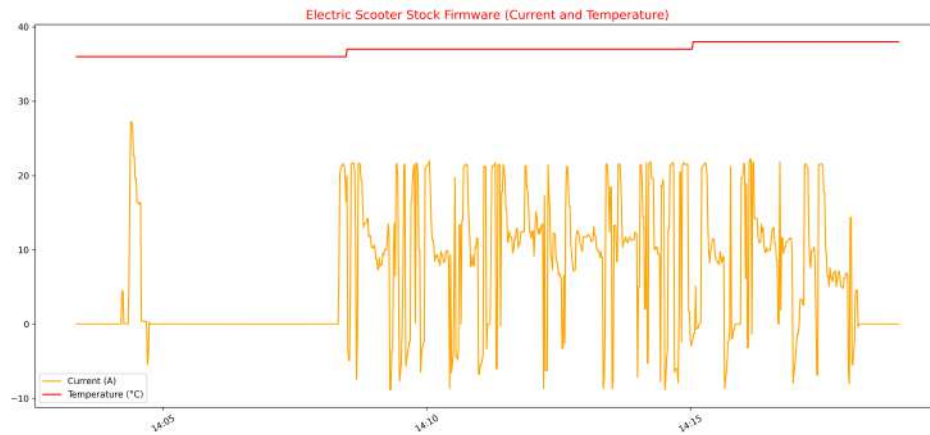
Figure 5.3. E-scooter, Current and temperature over time
