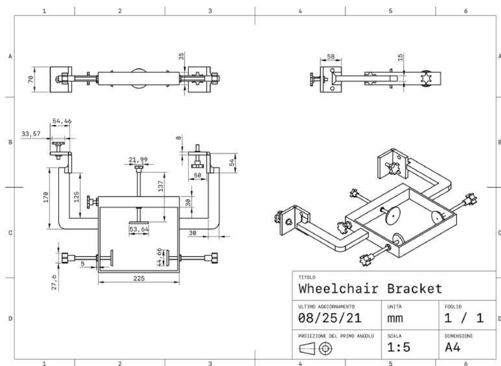
Figure D.1. 3D wheelchair bracket design
