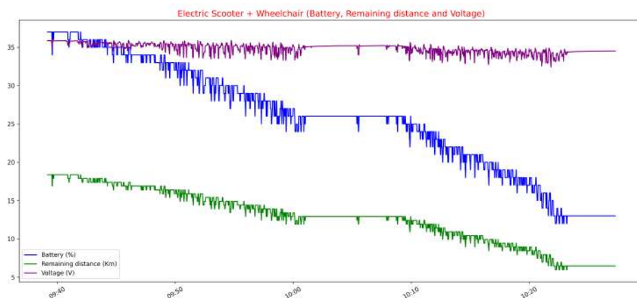
Figure 5.4. E-scooter + Wheelchair, Battery, remaining distance and voltage over time
