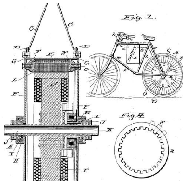
Figure 0.1. Ogden Bolton Jr.'s electric motorcycle patent from 1895
